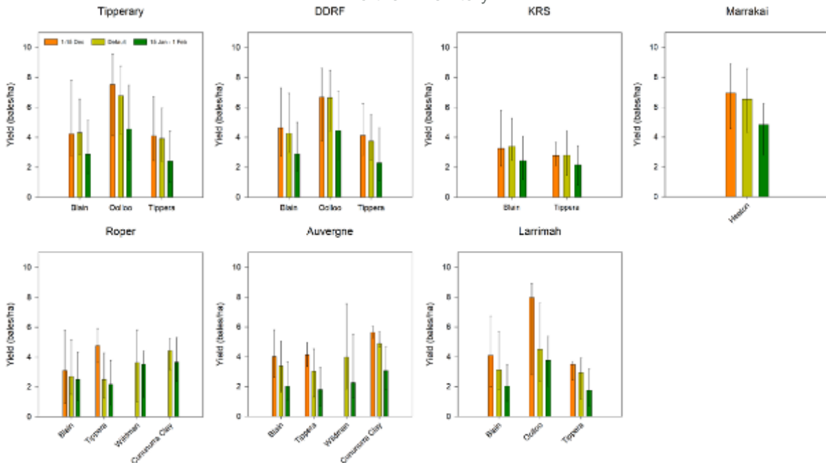
Fig. 2. 8 Simulated rainfed median cotton yields for 1957–2021 and their range (10 to 90% of seasons) within three planting windows 1–15 Dec (early), 15-Dec to 15-Jan (default) and 15-Jan to 1-Feb (late). Simulated yields are for a crop planted on the first day within the sowing window when planting was possible.
